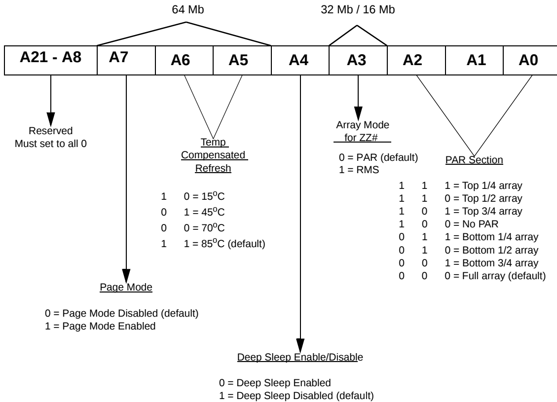
Figure 39. Mode Register
