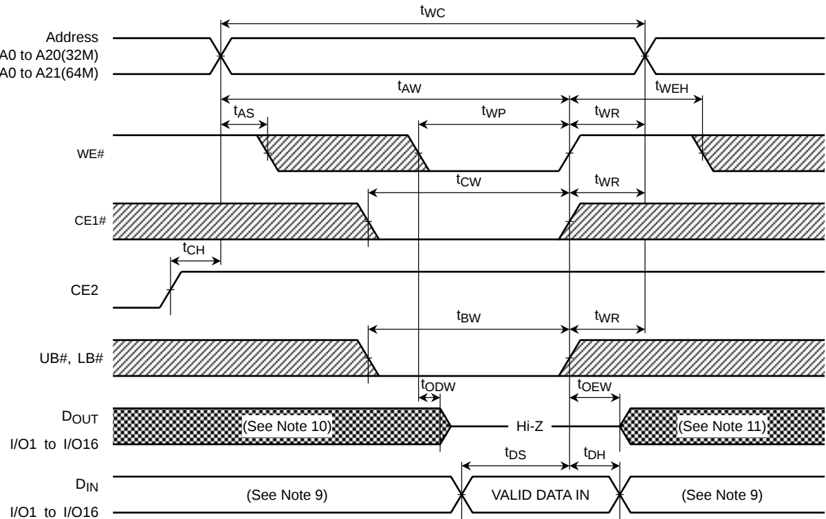
Figure 26. Write Cycle #1 ( \overline{WE\#} Controlled) (See Note 8)
