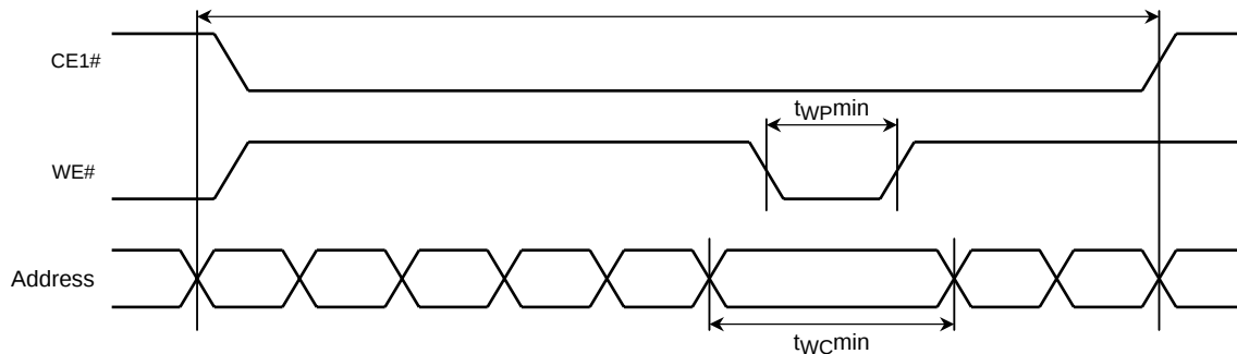
Figure 31. Write
