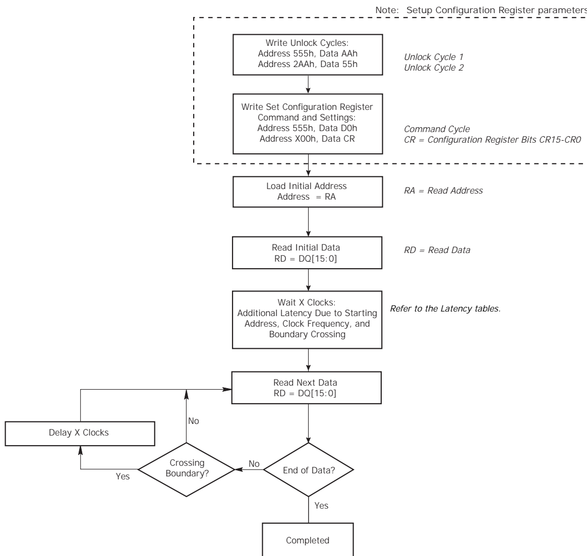
Figure 7.2. Synchronous Read
