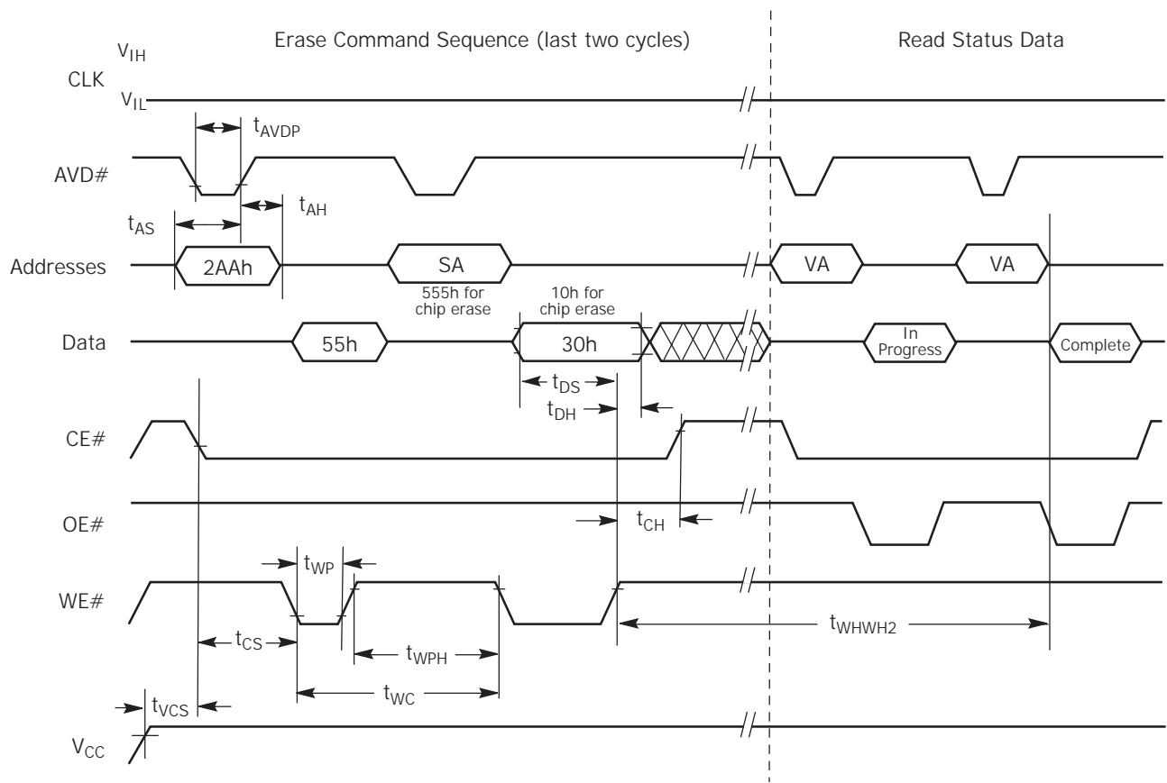
Figure II.I3. Chip/Sector Erase Operation Timings
