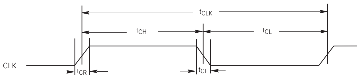
Figure II.6. CLK Characterization
