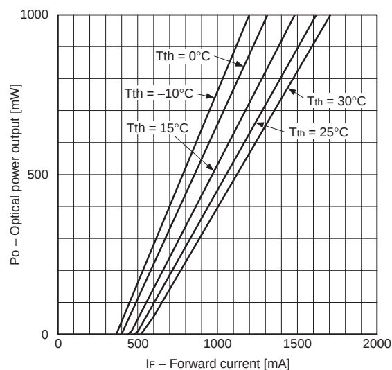
Optical power output vs. Forward current characteristics
