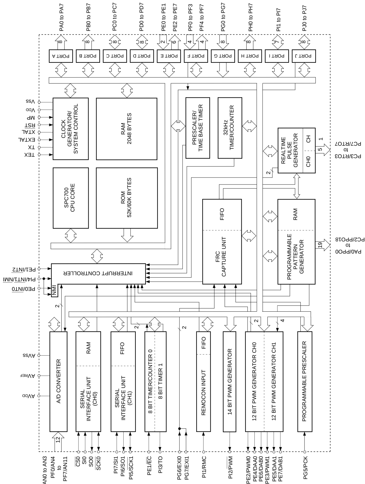
Block Diagram
