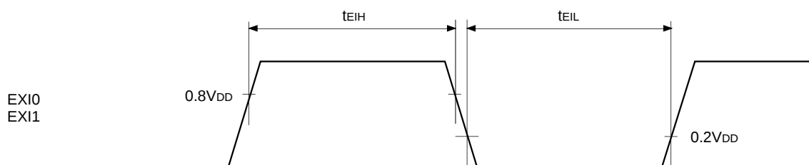
Fig. 10. Other timings
