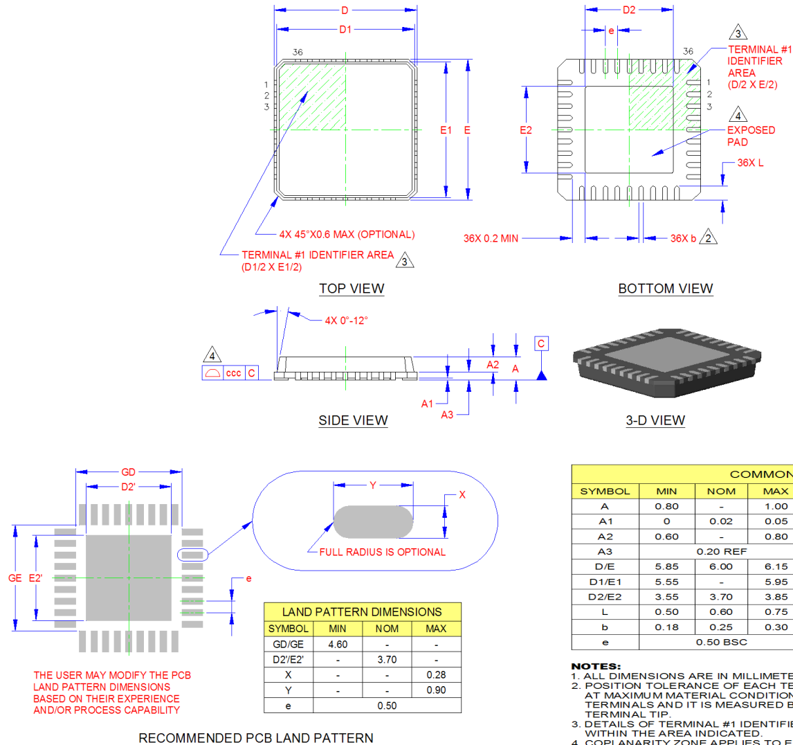
Figure 7.1 36-Pin QFN, 6x6mm Body, 0.5mm Pitch
