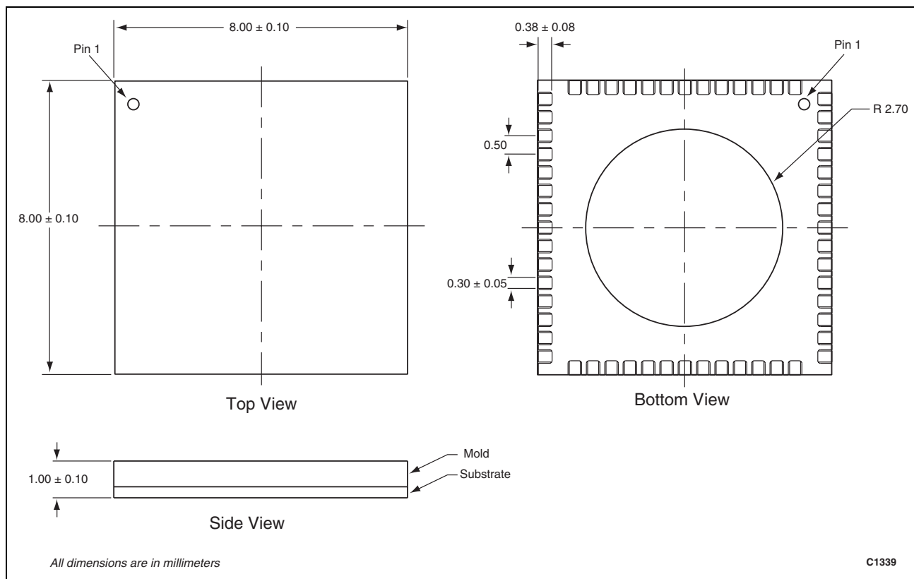
Figure 28. CX74063-26 56-Pin RFLGA Package Dimension Drawing
