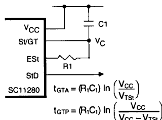
Figure 3. Basic Steering Circuit
