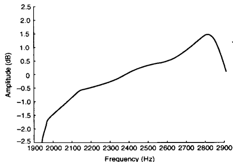
Figure 5. High-Band Response—Normalized
