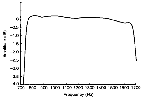
Figure 3. Low-Band Response—Normalized
