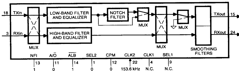
Figure 11. V.22 Originate Mode
