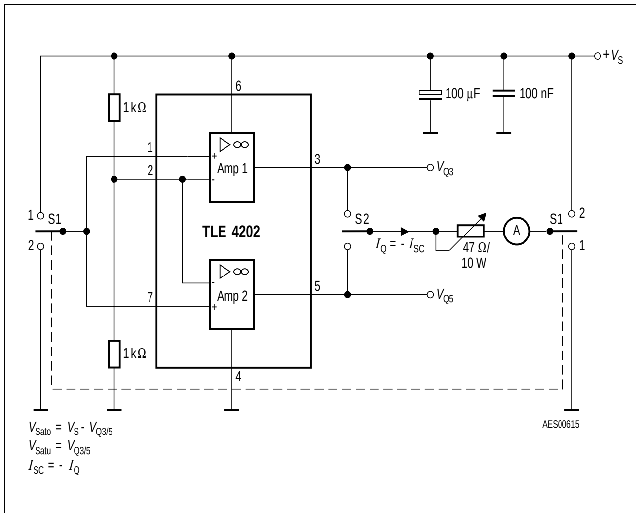
Figure 4 Test Circuit 2
