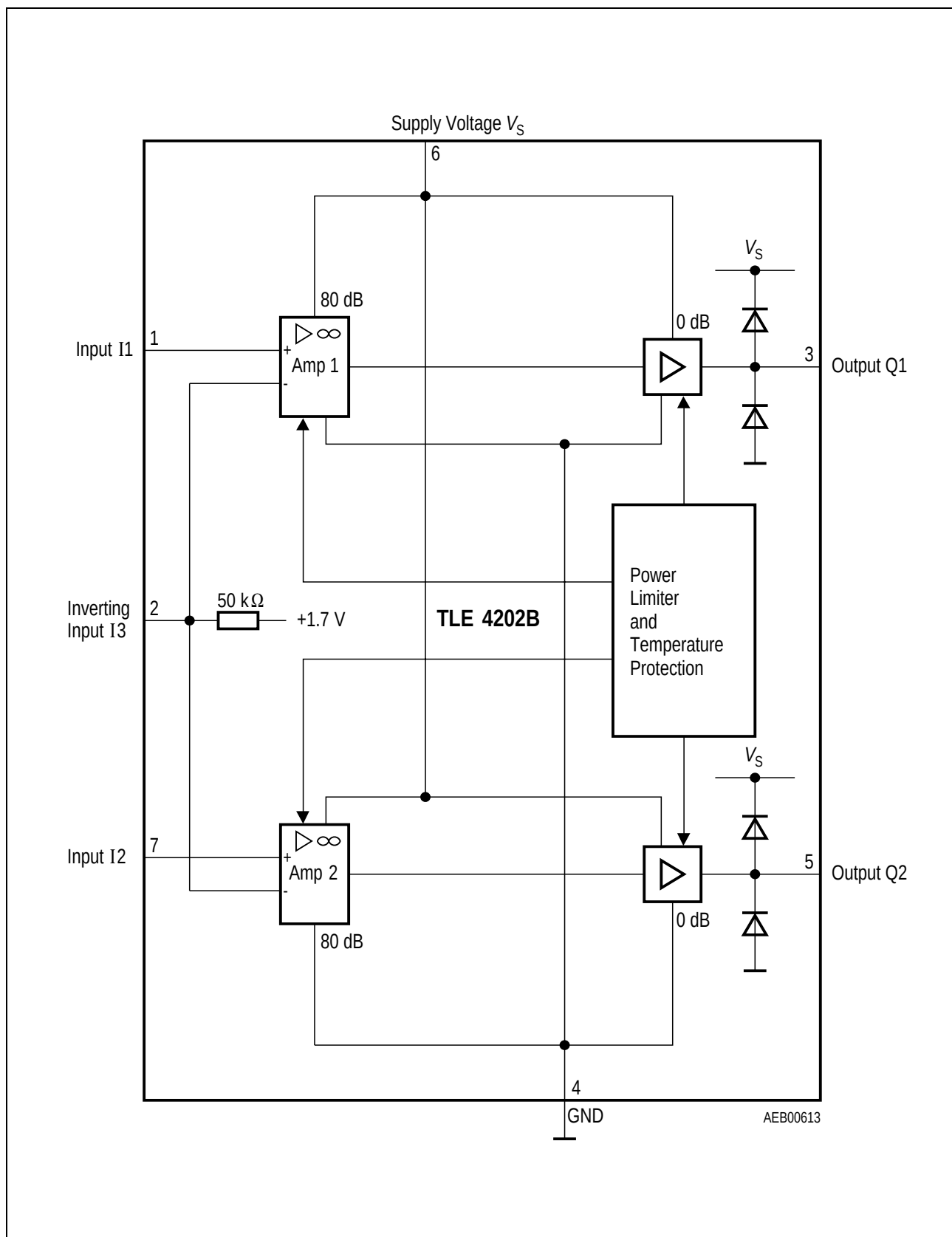
Figure 2 Block Diagram
