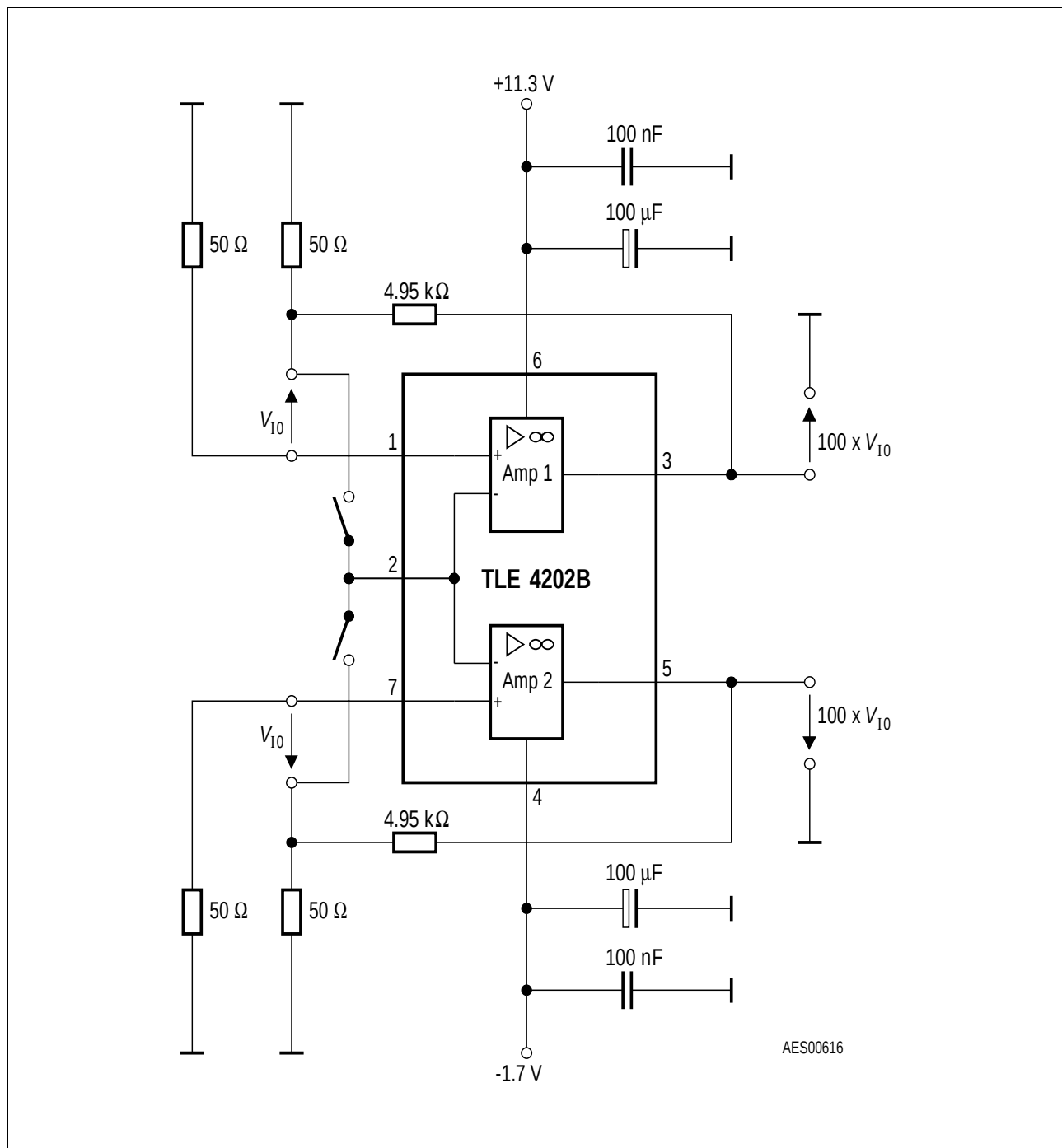
Figure 5 Test Circuit 3
