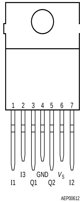
Figure 1 Pin Configuration (top view)
