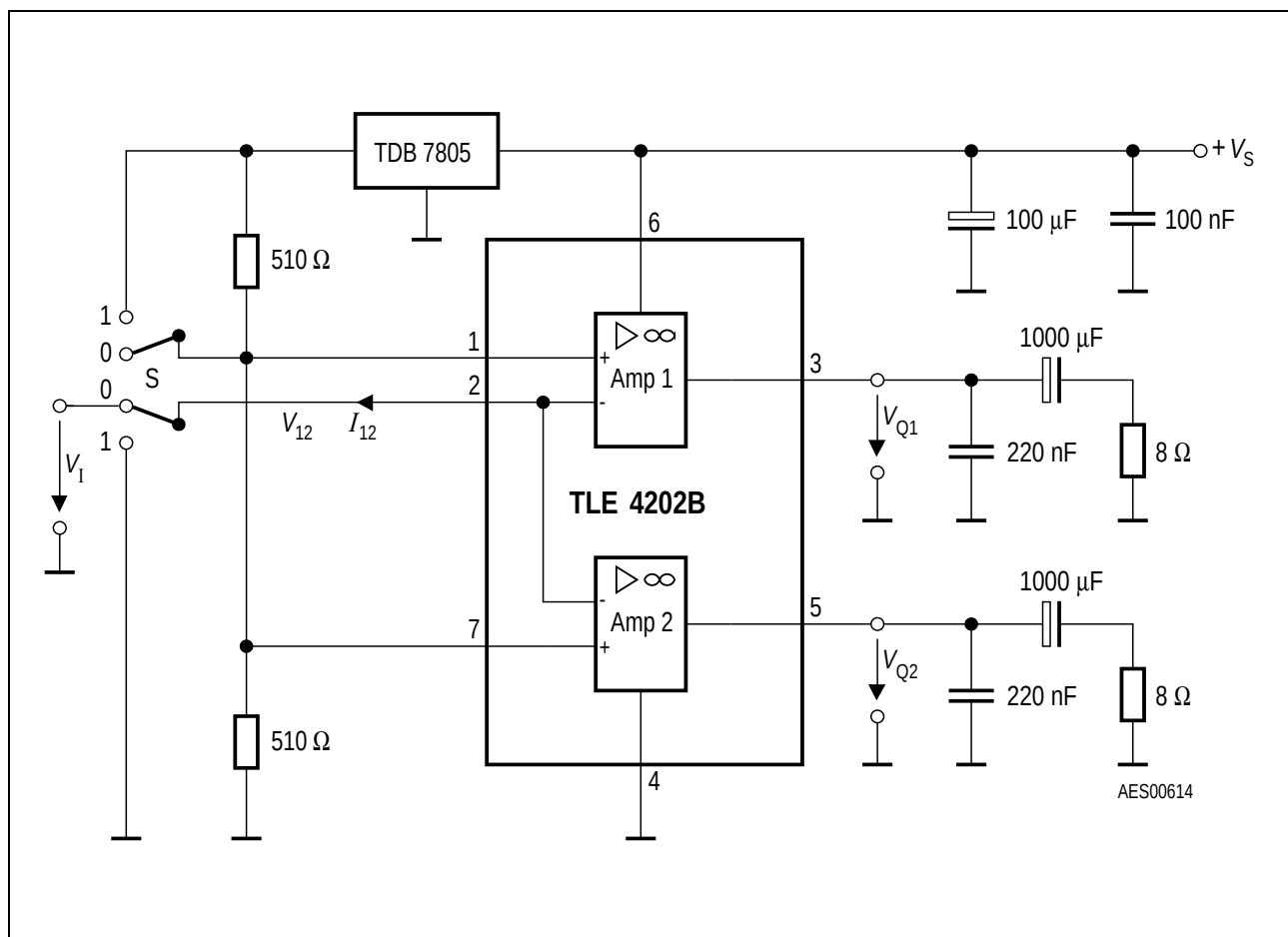
Figure 3 Test Circuit 1
