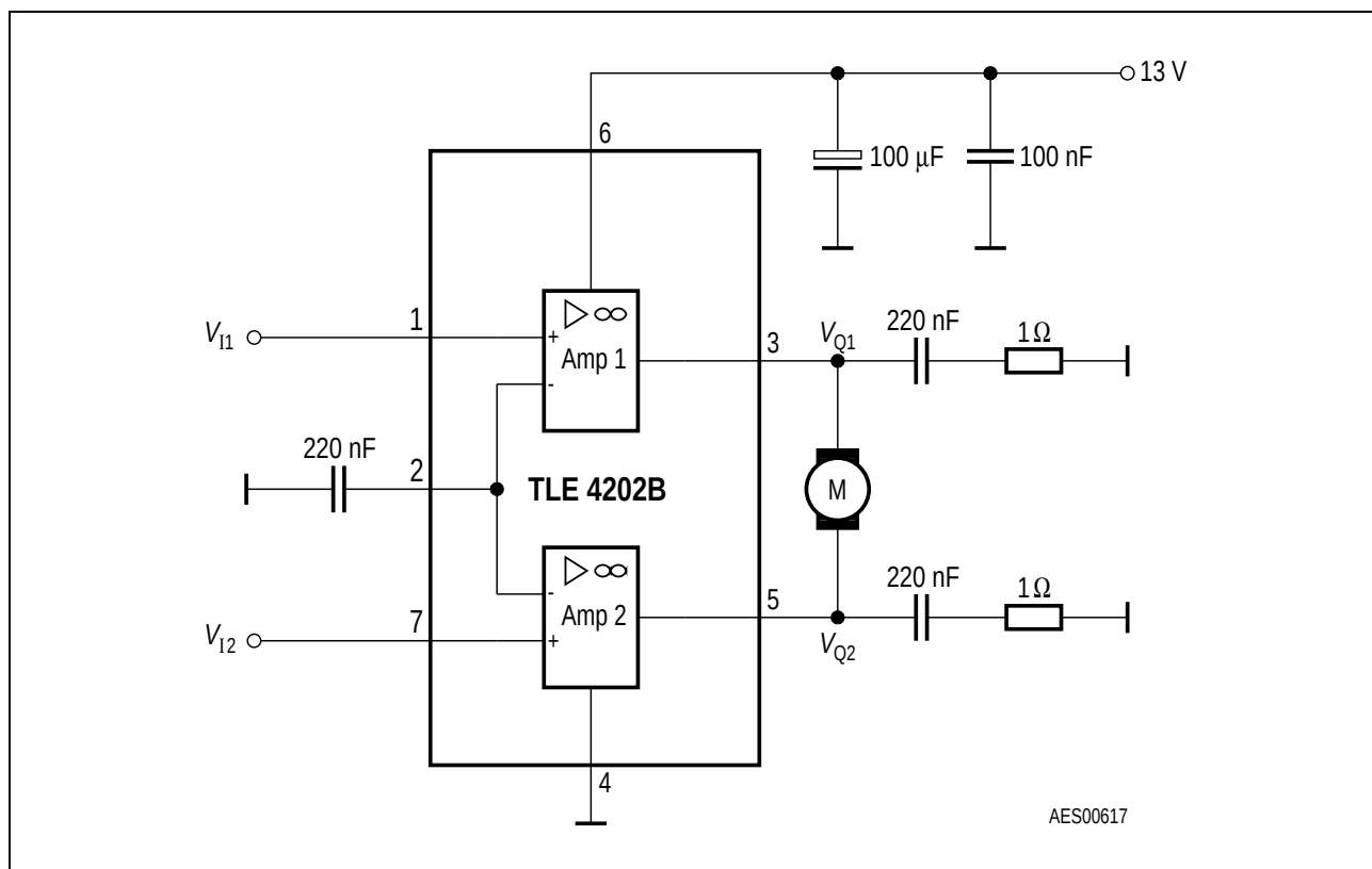
Figure 6 Application Circuit
