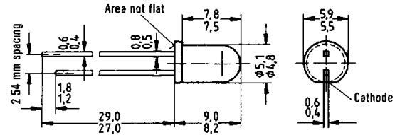
Package Dimensions mm
