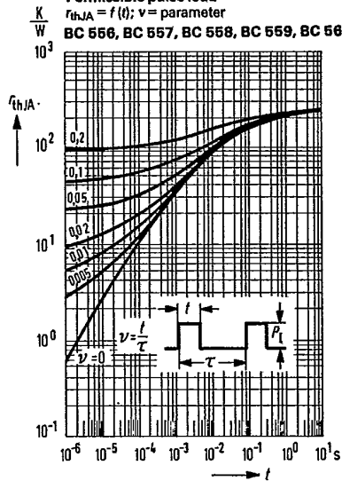
Permissible pulse load r_{\text{thJA}} = f(t) ; v = \text{parameter}
