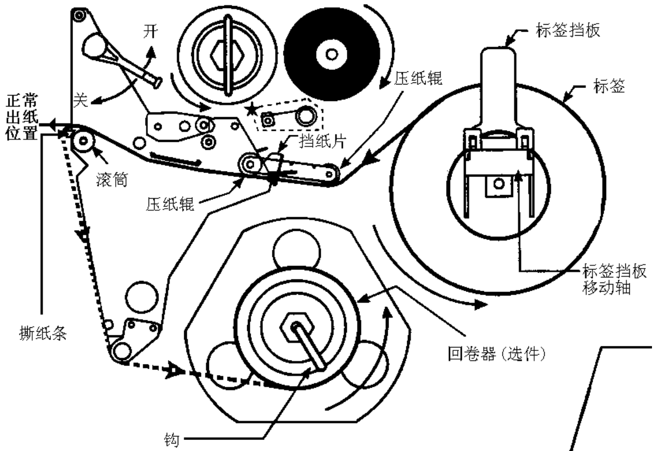
[标签安装图]
