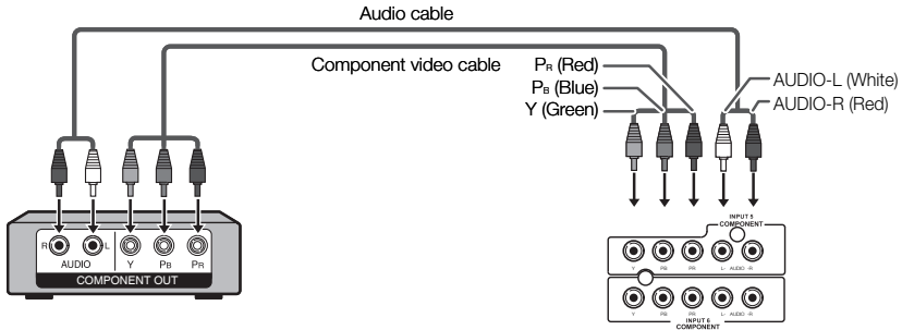
Back panel horizontal inputs
