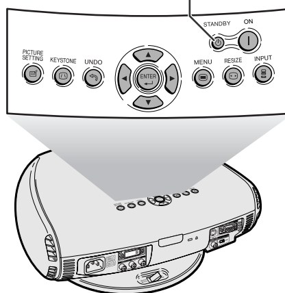
STANDBY button
