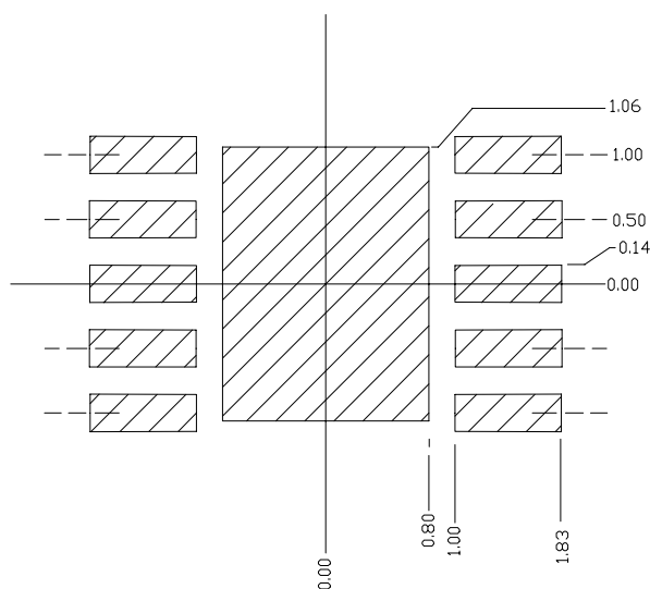
SUGGESTED PCB LAND PATTERN
