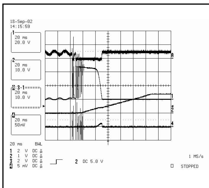
Figure 7. Start-up with no load.
