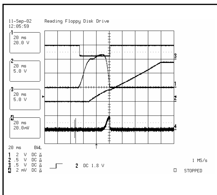
Figure 3. Start-up with no load.
