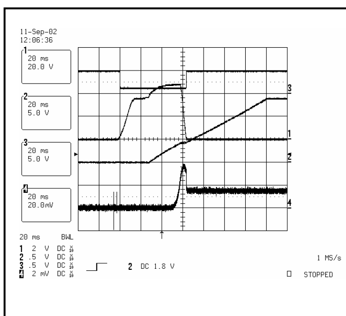
Figure 4. Start-up with 1A load.
