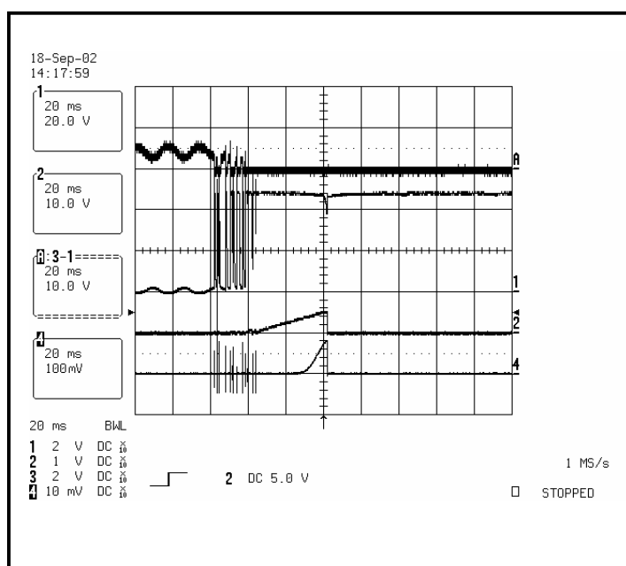
Figure 9. Start-up with “over the limit” load.
