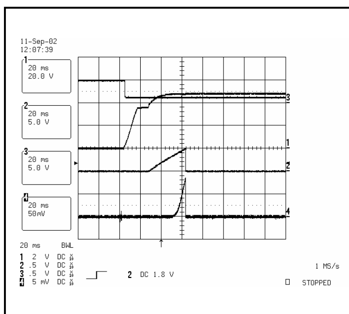
Figure 5. Start-up with "over the limit" load.
