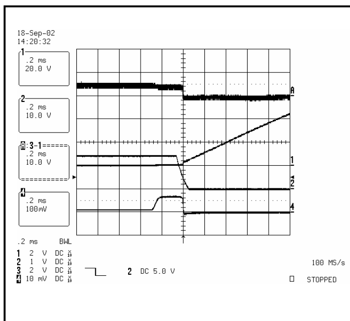
Figure 10. Over-current/Short circuit.
