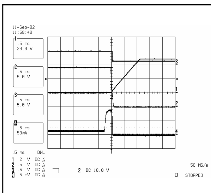
Figure 6. Over-current/Short circuit.
