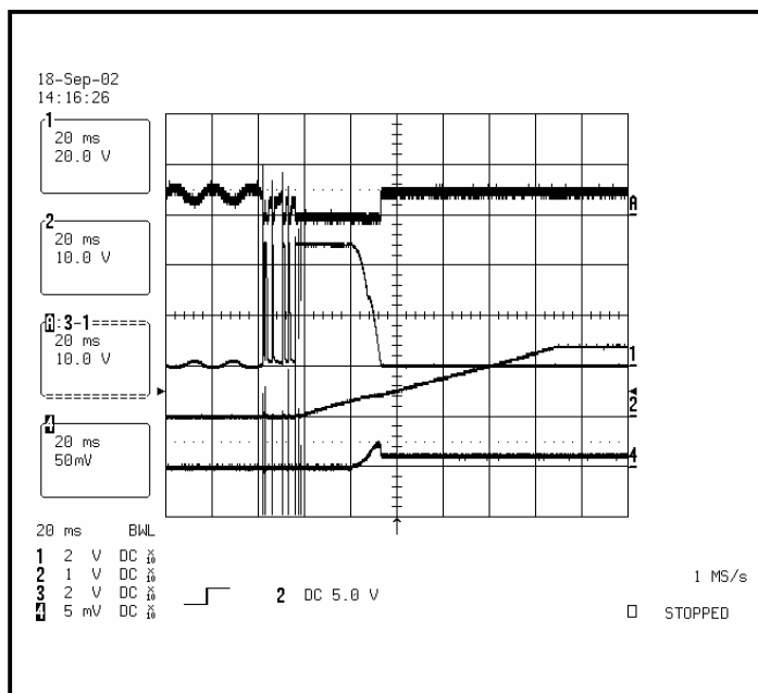
Figure 8. Start-up with 1A load.
