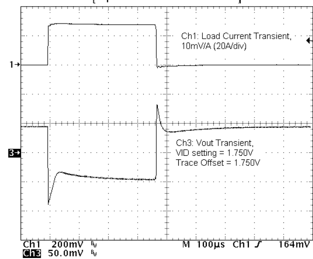
Transient Response Vo=1.75V, Io=0A to 28A
