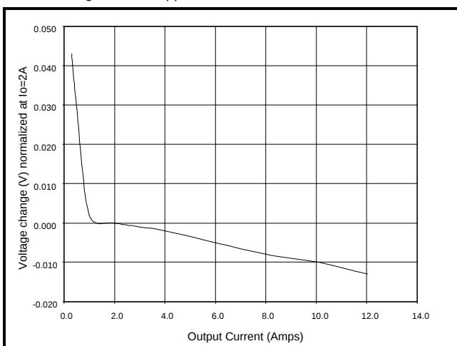
SC1150 Regulation in Application circuit 16935E
