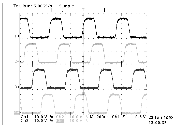
Fig. 1: The four Gate Drives firing 90° out of phase. V_{\text{OUT}} = 2.0\text{V} , I_{\text{OUT}} = 10\text{A}
