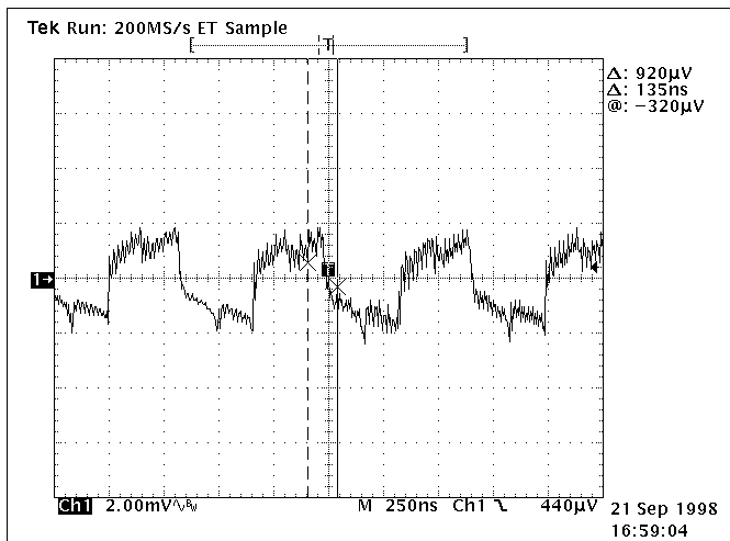
Fig. 4: V_{\text{OUT}} Ripple, V_{\text{OUT}} = 2.0\text{V} , I_{\text{OUT}} = 30\text{A}
