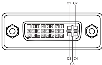
Pin Configuration
