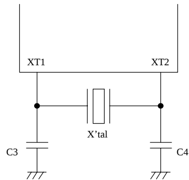
Figure 2 Crystal oscillation
