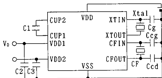
Figure 5 Output Voltage Test Circuit
