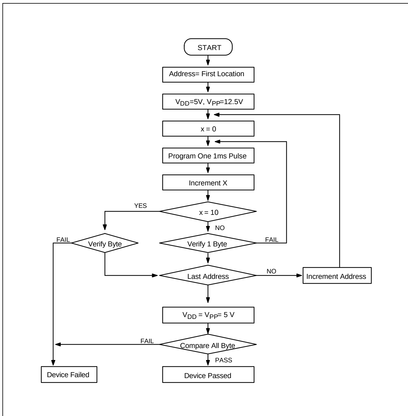
Figure 15-5. OTP Programming Algorithm
