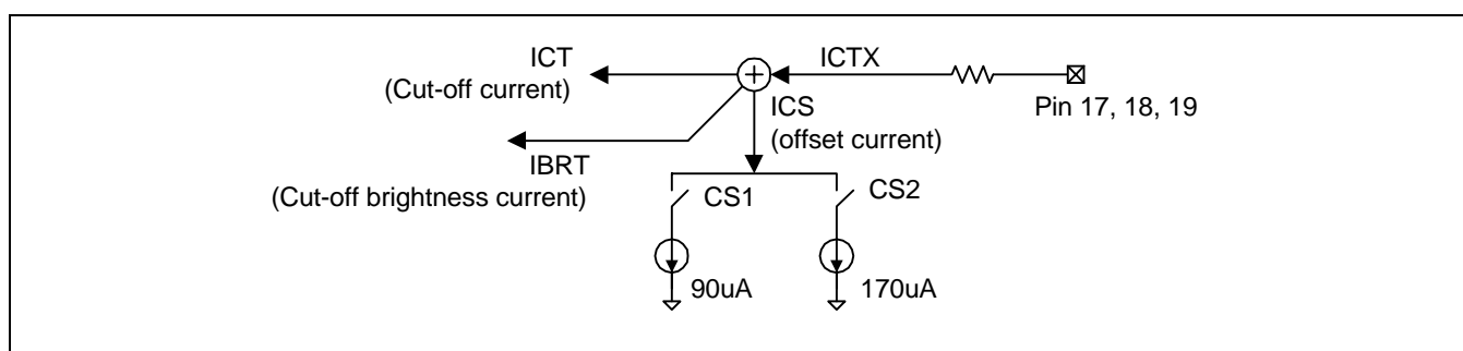
Figure 4. Internal Diagram
