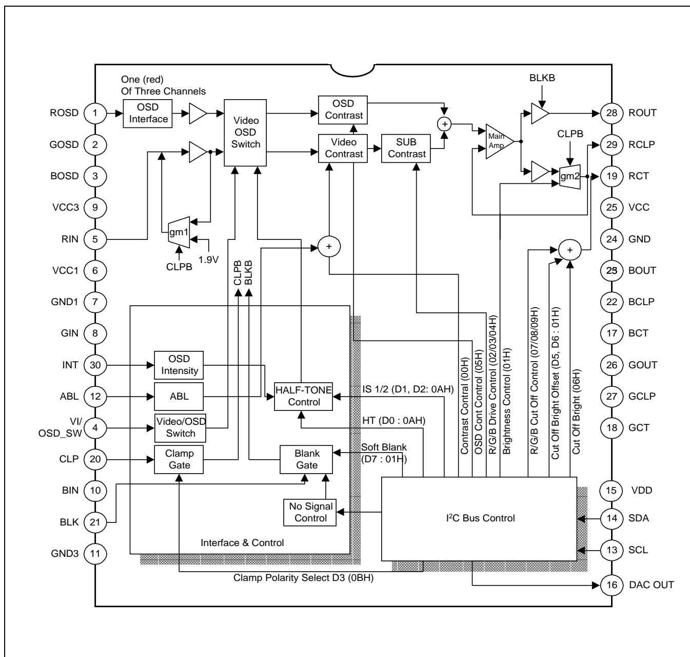
Figure 1. Block Diagram
