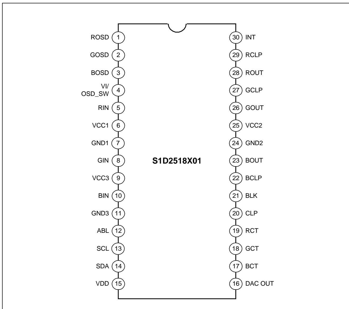
Figure 2. Pin Configuration
