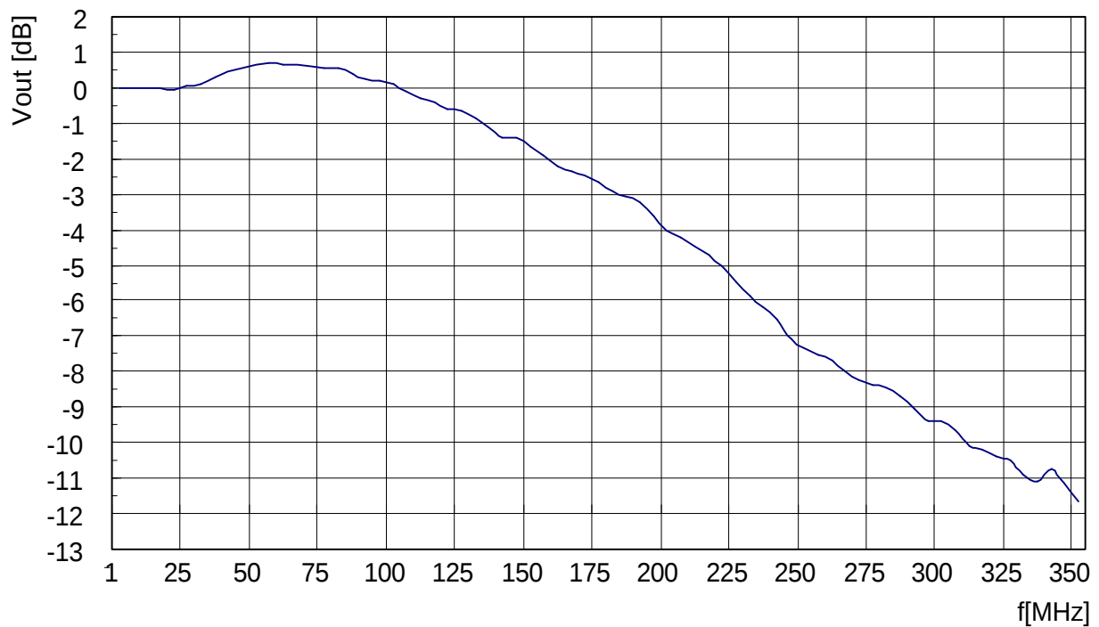
f-3dB (Video Preamp)
