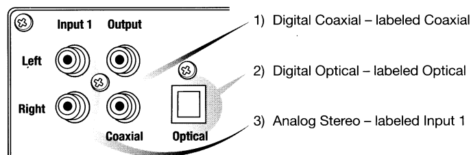
Rear input panel of ZVOX 575 HSD
