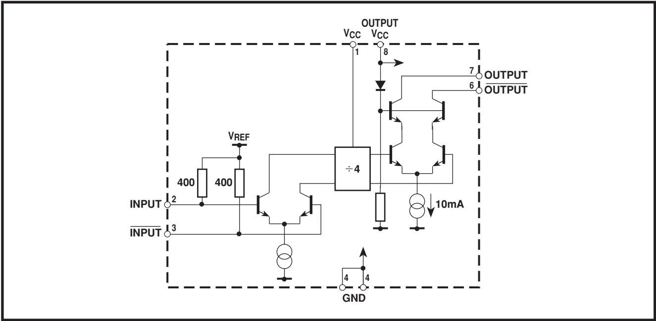
Figure 1 block diagram
