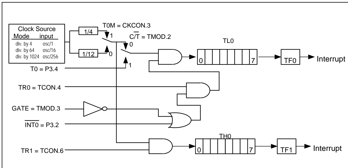
Figure 13. Timer/Counter 0 Mode 3
