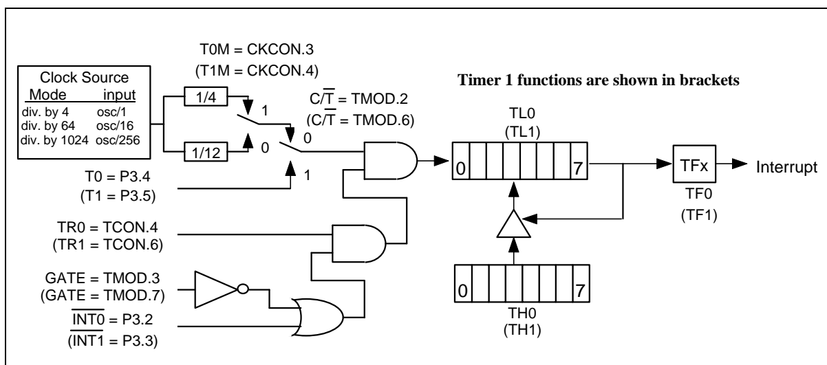
Figure 12. Timer/Counter Mode 2.
