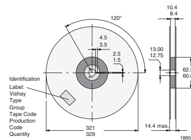
Figure 11. Reel dimensions - GS18
