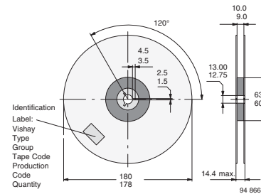
Figure 10. Reel dimensions - GS08
