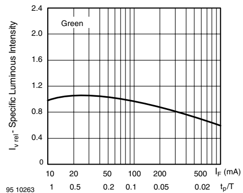
Figure 6. Specific Luminous Intensity vs. Forward Current
