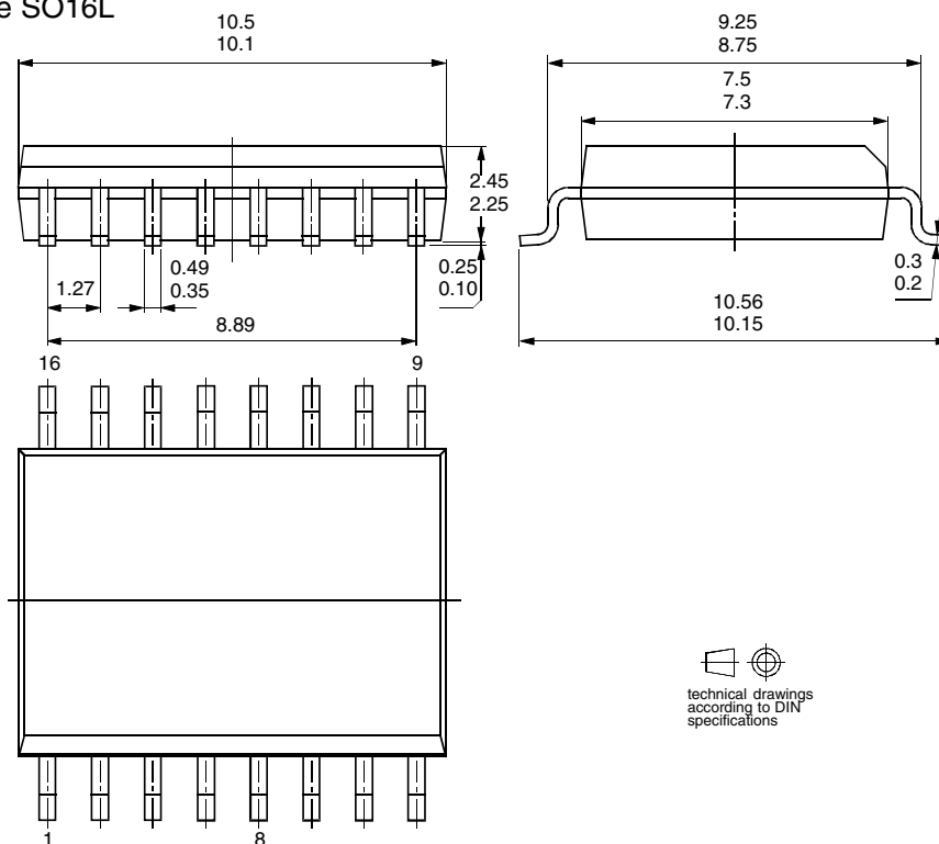
Package SO16L
