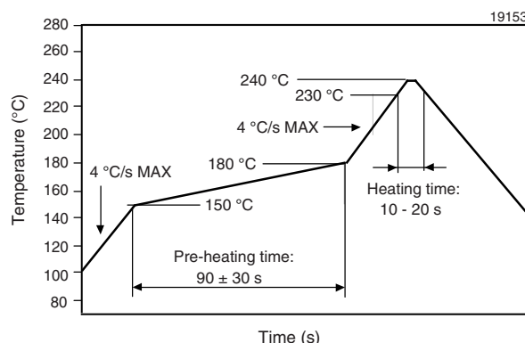
Figure 14. Lead Tin (SnPb) Reflow Solder Profile
