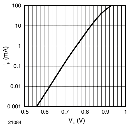
Figure 3. Typical Forward Current I_F vs. Forward Voltage V_F
