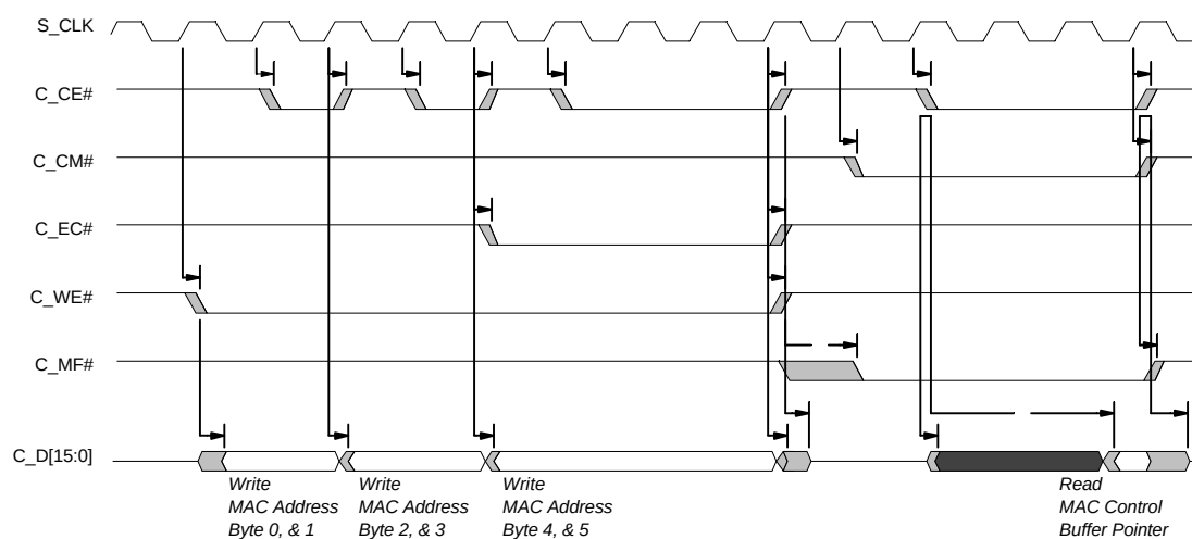
Typical MAC Address Compare Operation
