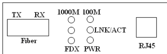
Figure 1 - M7260A Front Panel
