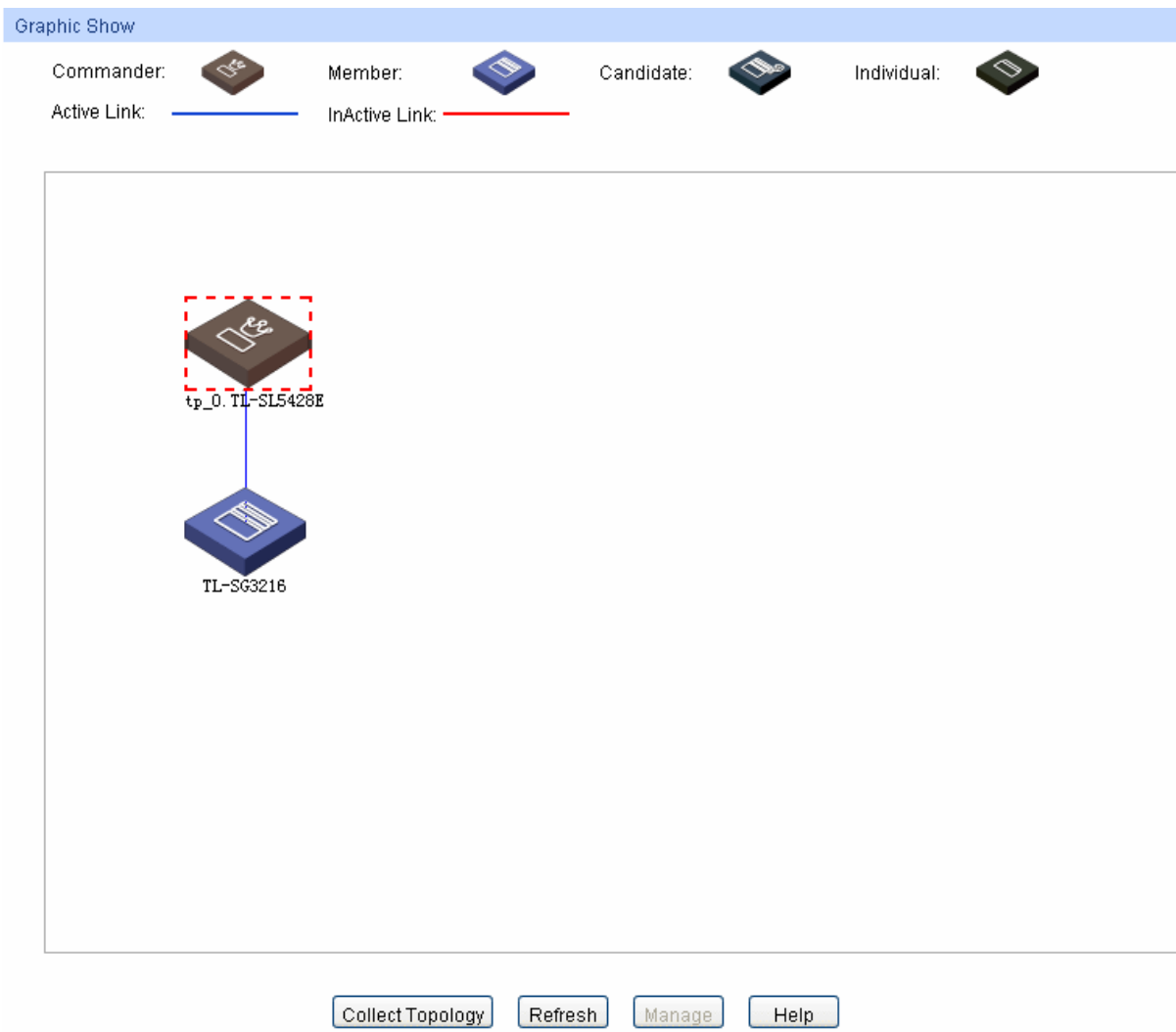
Figure 13-18 Collect Topology
