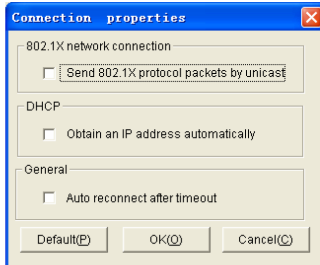
Figure C-12 Connection Properties
