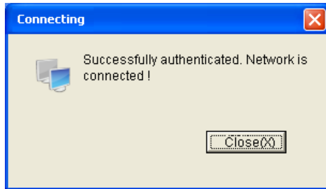
Figure C-14 Successfully Authenticated
