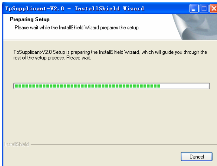
Figure C-8 Preparing Setup
