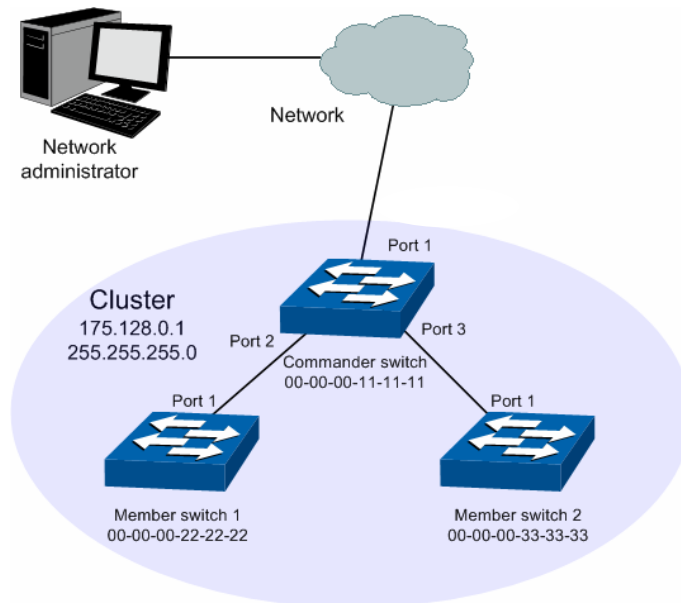
Figure 13-19 Network diagram
