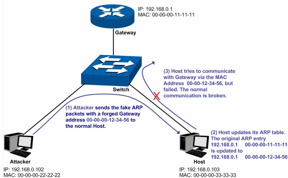
Figure 11-9 ARP Attack - Imitating Gateway
