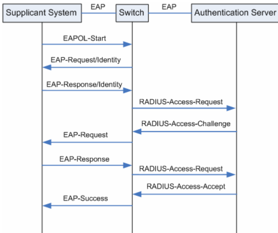
Figure 11-20 EAP-MD5 Authentication Procedure
