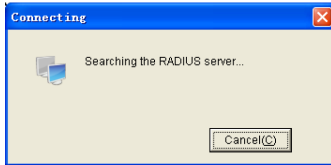
Figure C-13 Authentication Dialog
