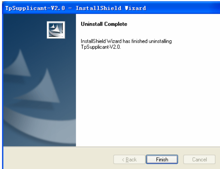
Figure C-10 Uninstall Complete
