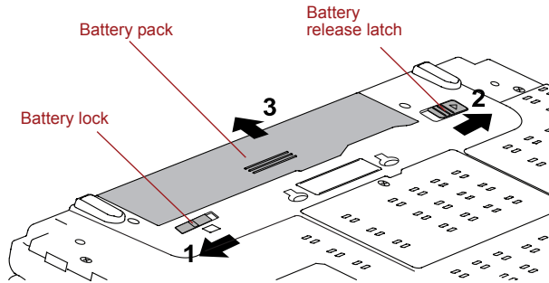
Figure 6-1 Releasing the battery pack
