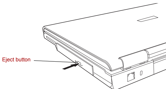
Pressing the eject button
