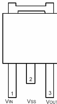
TO-252 (TOP VIEW)
