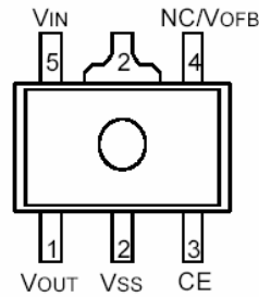
SOT-89-5 (TOP VIEW)
