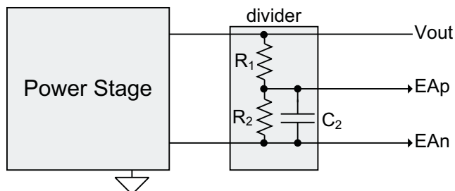
Figure 16. EAp/EAn Input Network
