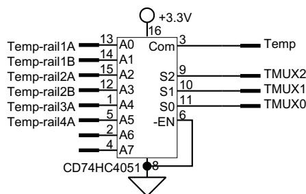
Figure 12. Temperature Mux (4-rail, 6-phase Example)
