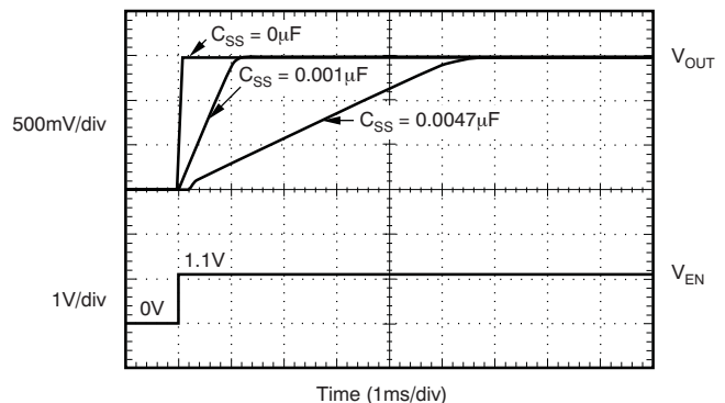
Figure 2. Turn-On Response
