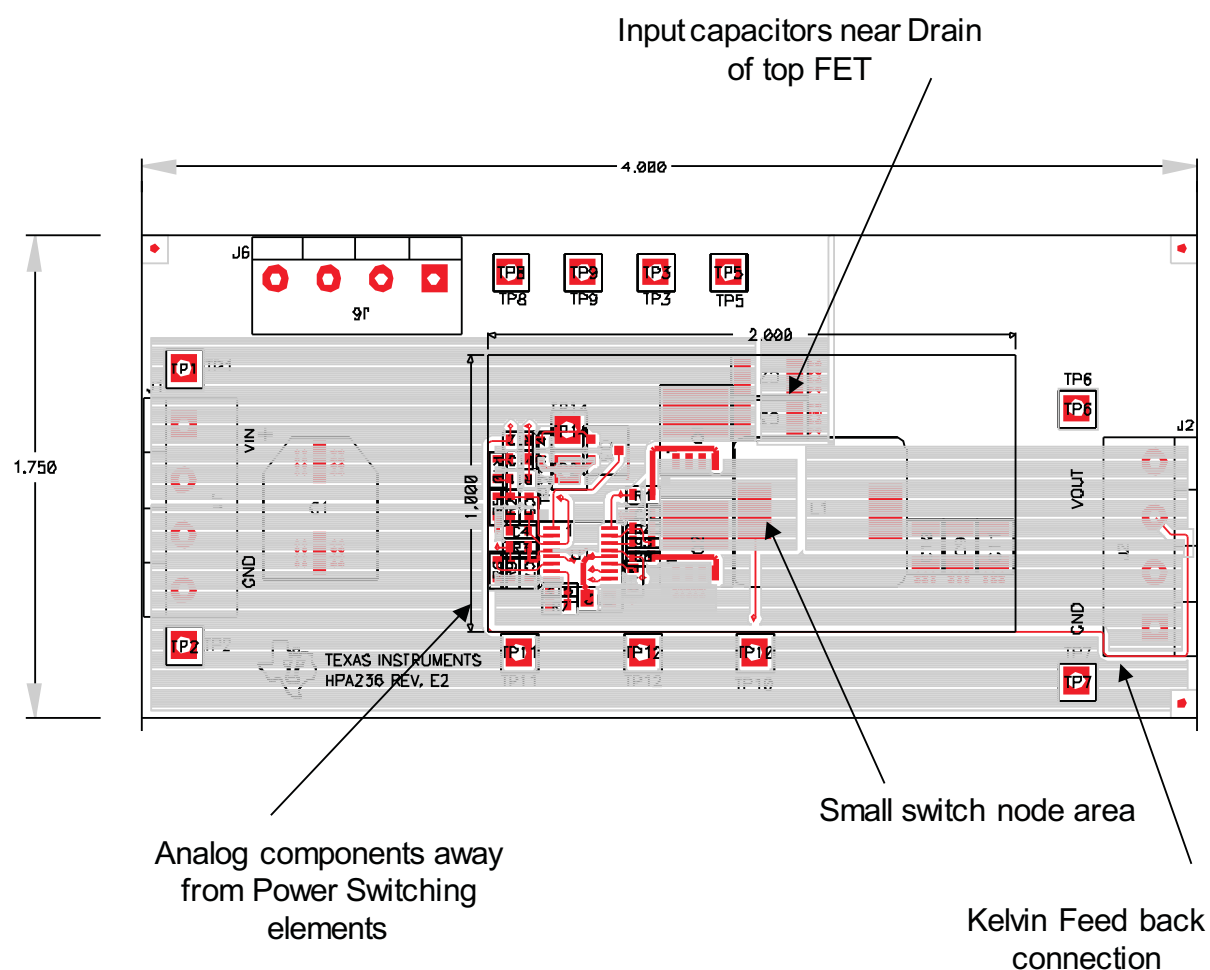
Figure 23. Board Layout
