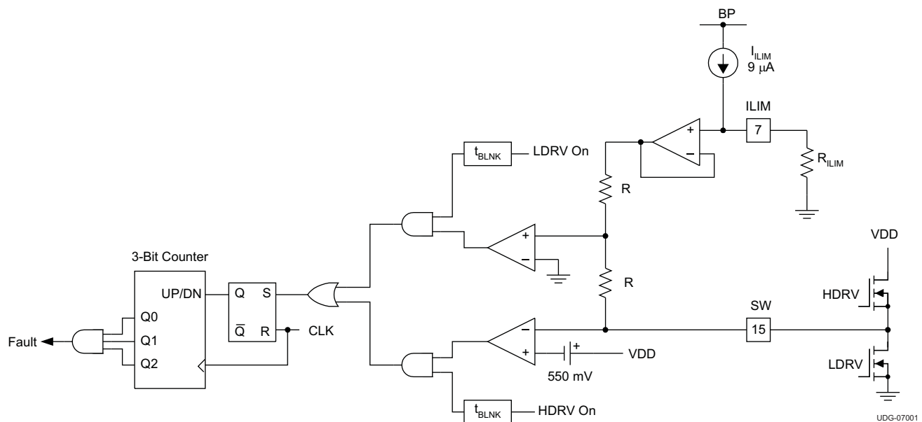
Figure 21. Overcurrent
