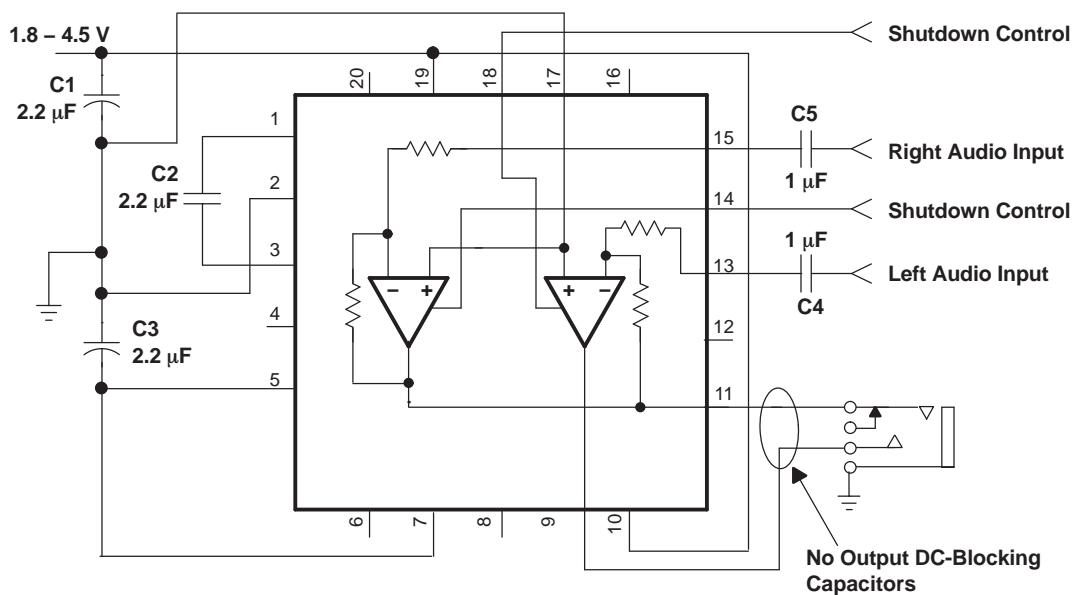
Figure 77. Typical Circuit
