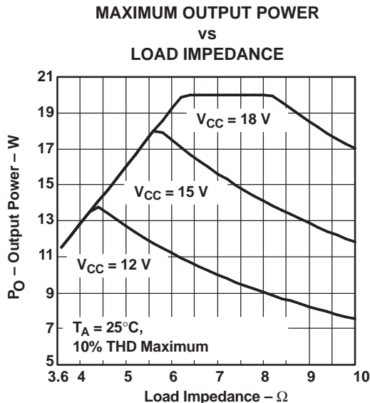
Figure 33. Output Power
