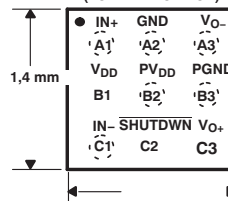
9-BALL WAFER CHIP SCALE, YZF PACKAGE, (TOP VIEW OF PCB)
