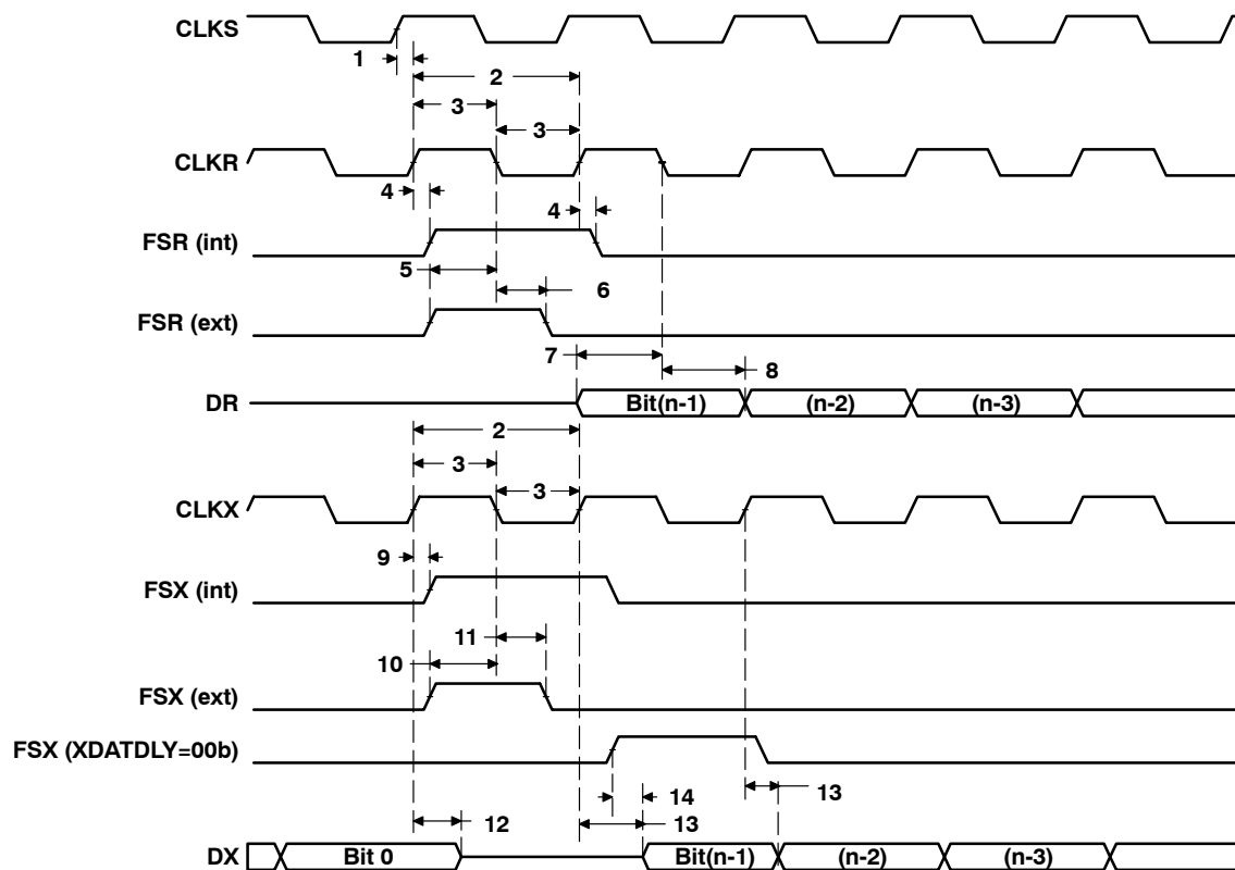
Figure 57. McBSP Timings
