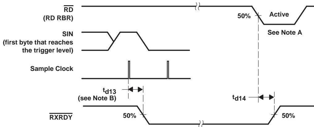
Figure 10. Receiver Ready ( \text{RXRDY} ) Waveforms, \text{FCR0} = 0 or \text{FCR0} = 1 and \text{FCR3} = 0 (Mode 0)
