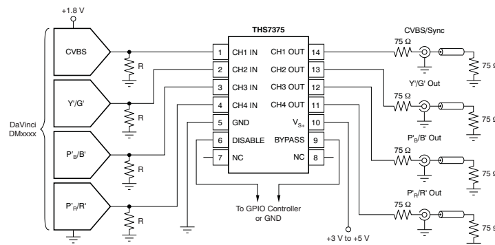
Figure 1. 3.3-V Single-Supply, DC-Input/DC-Output Coupled Video Line Driver
