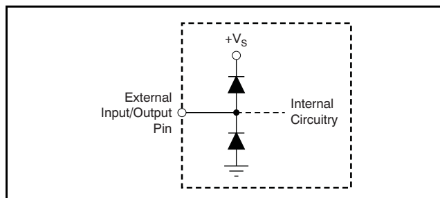
Figure 45. Internal ESD Protection
