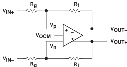
Diagram For Input Common-Mode Range Equations Figure 77
