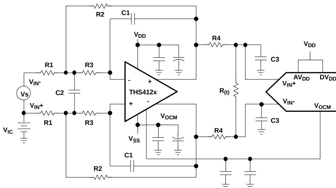
Figure 22. Antialias Filtering
